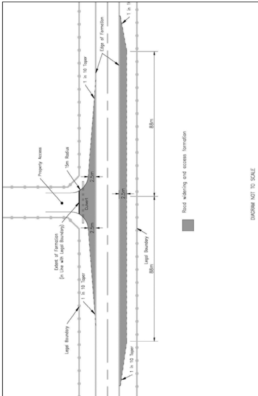
DIAGRAM TI-4 – RURAL PRIVATE ACCESS WITH FREQUENT HEAVY VEHICLE USE
